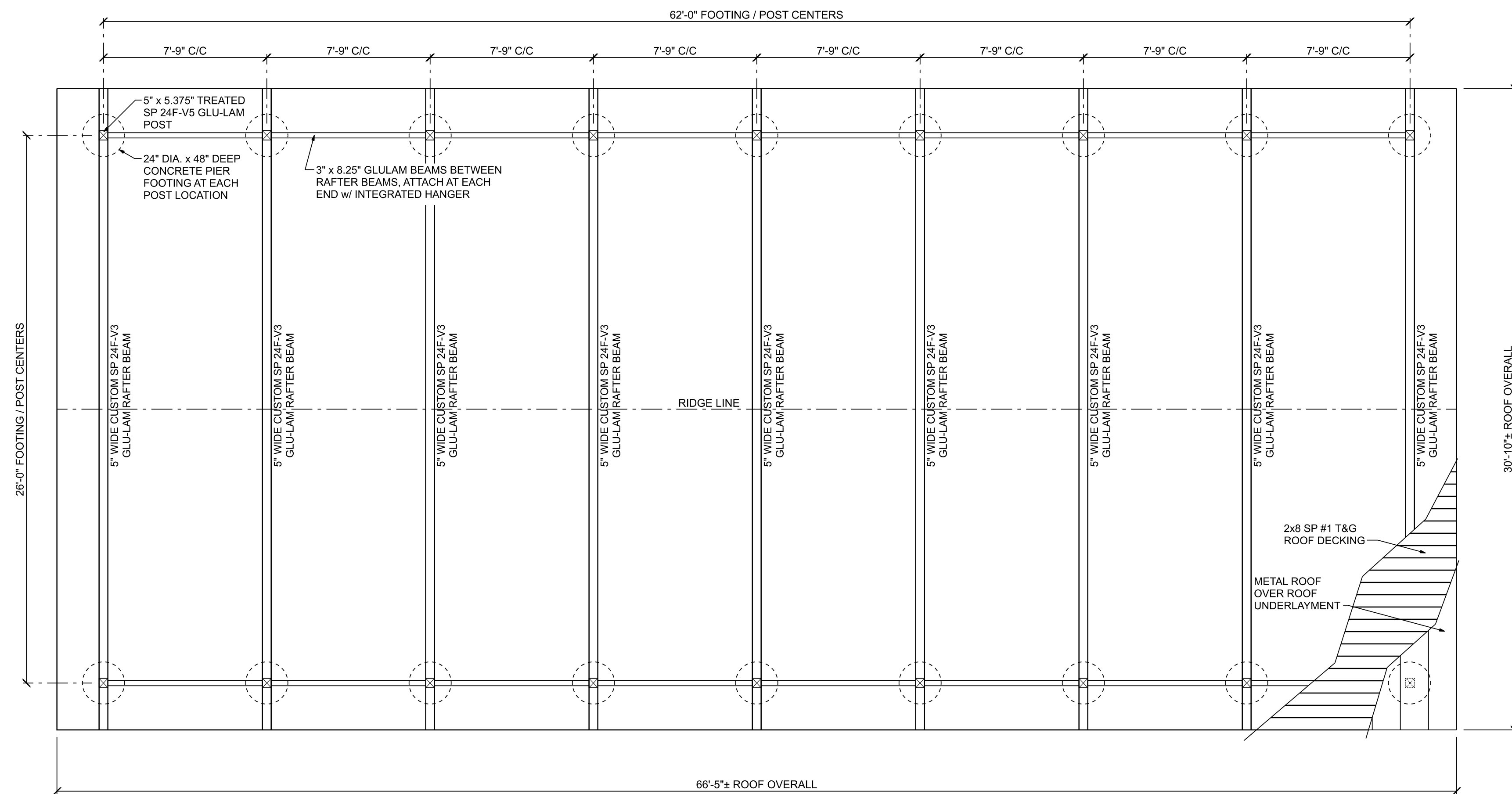
PLAN VIEW
