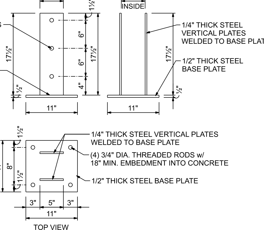
STEEL POST BRACKET DETAIL NO SCALE MATERIAL: POWDER-COATED STEEL
