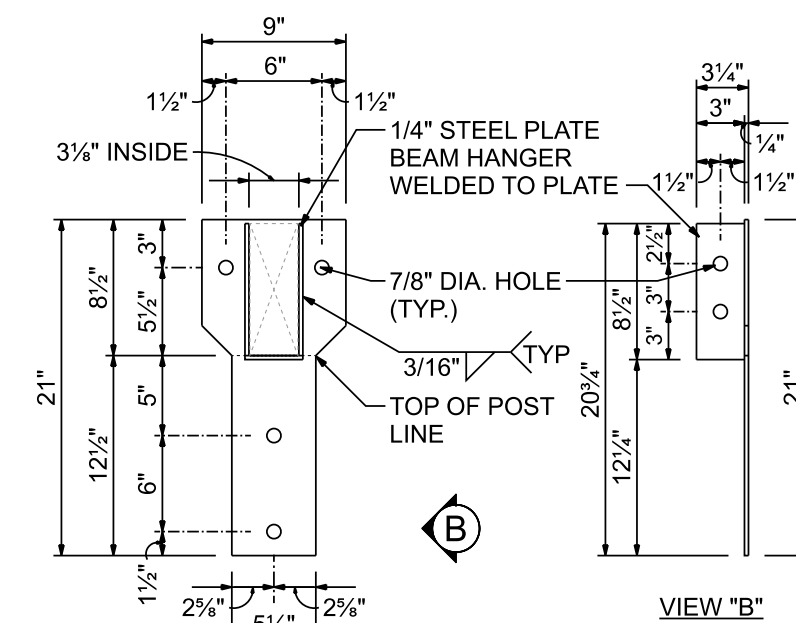
1/4" STEEL PLATE / HANGER DETAIL SCALE: 1" = 1'-0"
